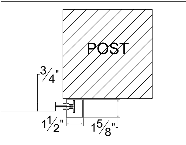
SIDE TRACK DETAIL
